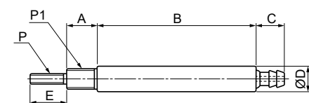
杆端无螺纹 Non-threaded rod end
