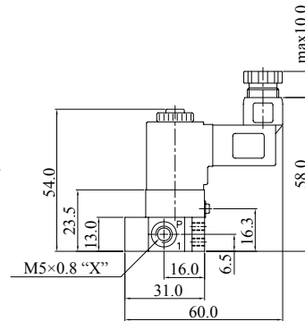
KSV211-D/DZ 常闭
